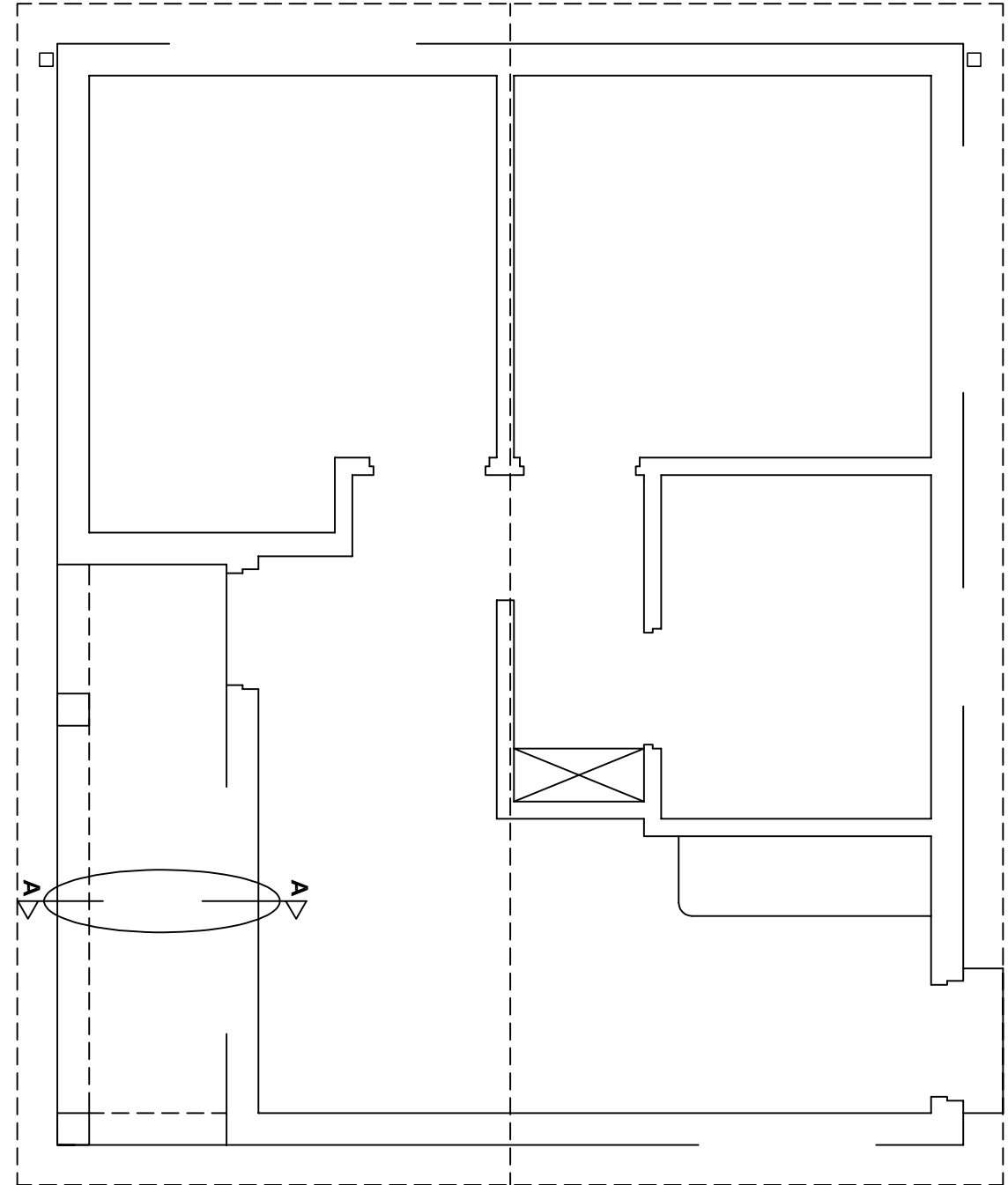
FLOORPLAN SCALE 1 : 50
